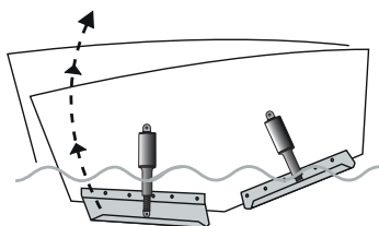
When the tabs are lowered, the water flow is redirected creating an upward force at the stern of the boat.
